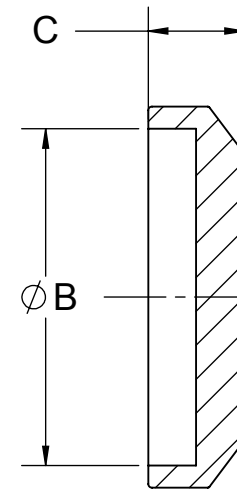
SECTION X-X
